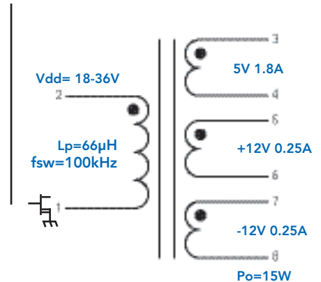
SCHEMATIC
