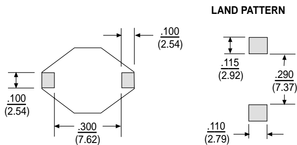
LAND PATTERN
